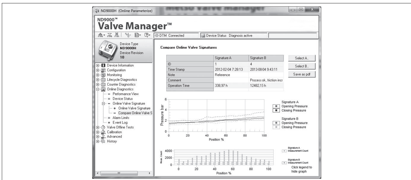
Fig. 2 Valve Online Signature feature shows friction of the control valve online, under normal process conditions when ever the valve is changing position.
