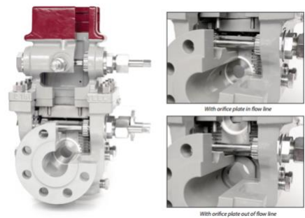
Double Chamber Orifice Fitting
